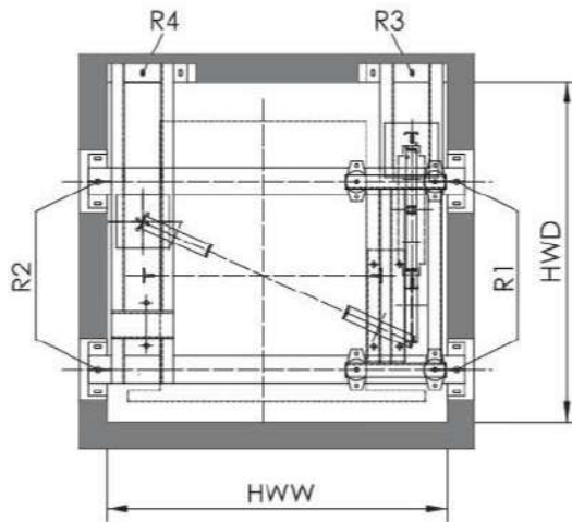
MACHINE PLAN
