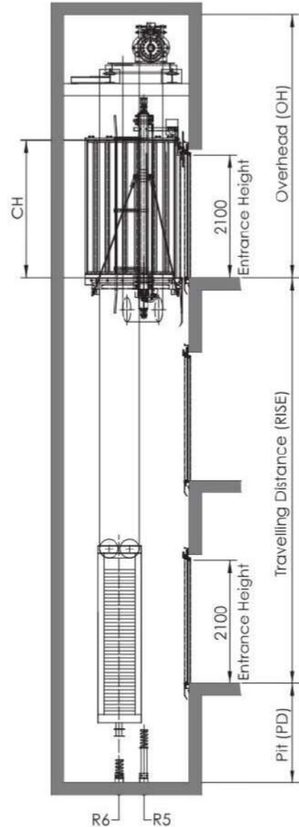
SECTION ELEVATION
