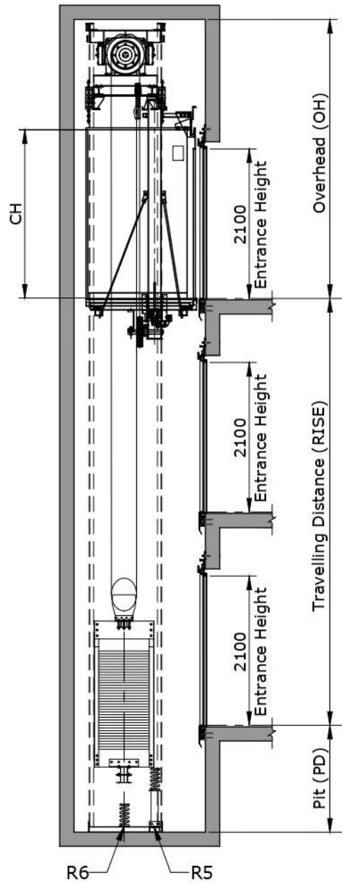
SECTION ELEVATION
