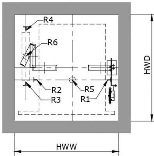
MACHINE PLAN
