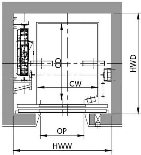
HOISTWAY PLAN
