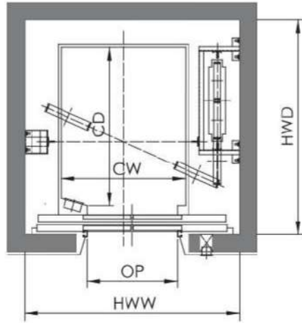
HOISTWAY PLAN
